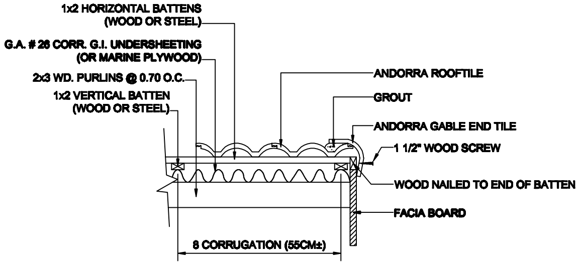
GABLE END TILE DETAIL SCALE 1:15 MTS.
